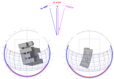
Sun Path Analysis
